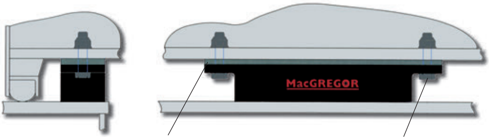
Adjusting plate
