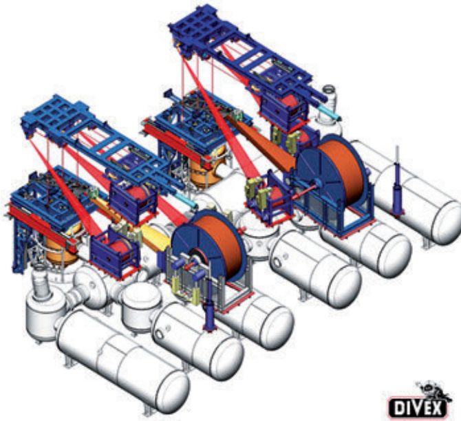
Diving system
