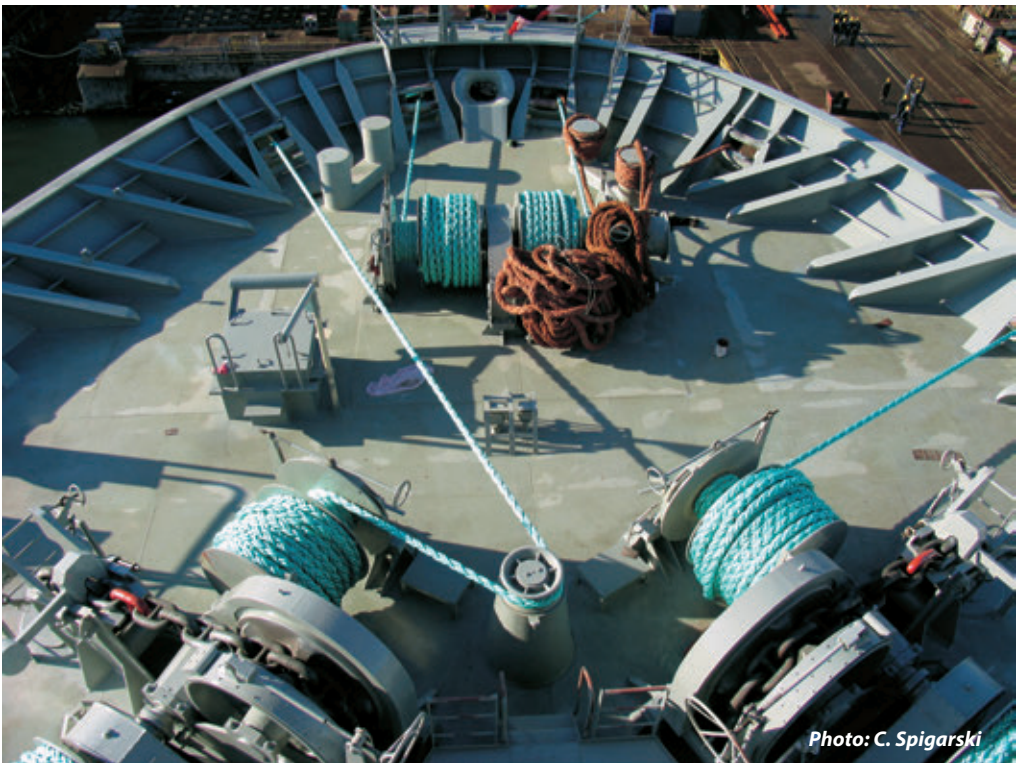
Anchor/mooring equipment on the forecastle deck of 4444 TEU vessel
