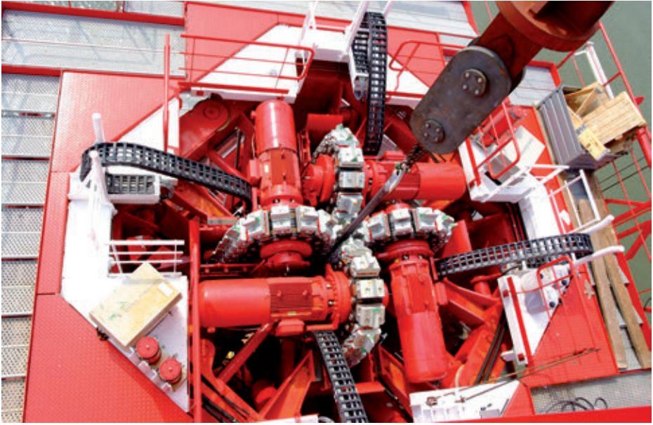
Pipe tensioner
