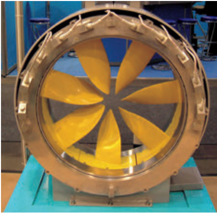
Rim drive thruster of EPS™ type from Van der Velden® Marine Systems
