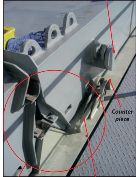
Double rubber lip sealing
