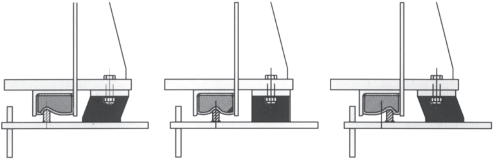
Flexipad flexes when the hatch cover and coaming move in the seaway
